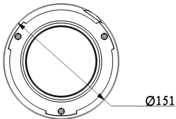
Figure 1-2 Dimension 2
